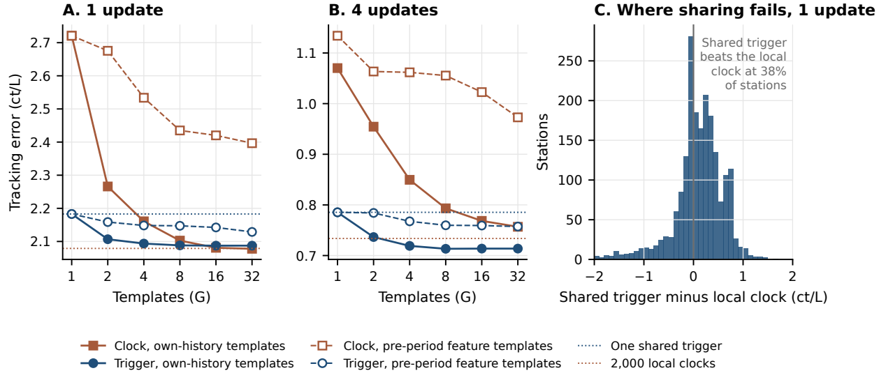
Figure 2: How much customization one shared trigger replaces. Panel A: full-year tracking error for libraries of G schedule templates or thresholds, with one permitted increase. Filled marks assign each station its own 2024-best template from a set chosen on the stations’ tuning losses; open marks assign templates from pre-period station features. The horizontal line is one shared trigger. Panel B: the same with four permitted increases; schedule templates are drawn from 200 locally tuned four-time schedules. Panel C: the distribution across 2,000 stations of shared-trigger minus local-schedule error with one permitted increase.
