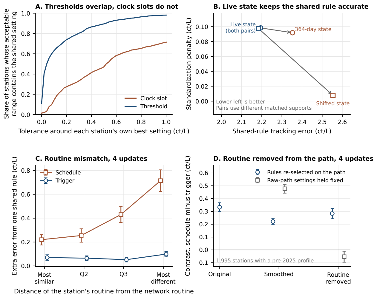
Figure 3: Why the shared trigger works. Panel A: share of stations for which the shared 2024 setting is within a stated error tolerance of the station's best 2025 setting, for thresholds and schedule times with one permitted increase. Panel B: shared-rule error and sharing penalty for triggers using the current, 364-day-lagged, or circularly shifted gap, evaluated on the same observations. Panel C: schedule and trigger sharing penalties by quartile of repricing-pattern distance at four permitted increases. Panel D: four-increase difference in sharing penalties on the original, smoothed, and de-cycled paths after retuning, and when the original settings are held fixed. Brackets are simultaneous 95 percent intervals within each analysis.
