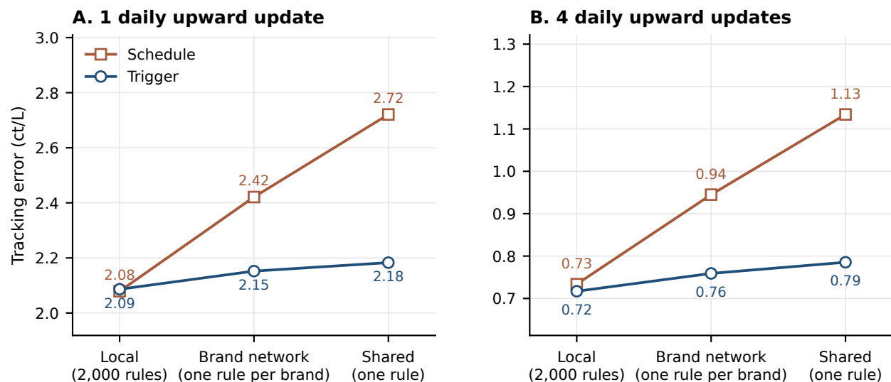
Figure 1: Tracking error as local rules are replaced by a brand-network rule and by one shared rule. Panels show one and four permitted daily increases under equal time weights. Schedule lines use squares; trigger lines use circles. Rules are selected using 2024 data and evaluated over full-year 2025 on 2,000 stations. The brand-network point tunes one rule within each of 16 recorded brand networks and pools the remaining stations.
